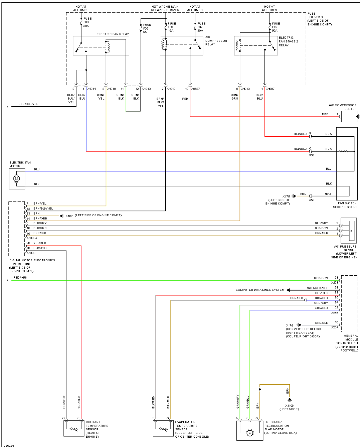
Fig. 2: Automatic A/C Circuit, W/ Dual Stage Cooling Fans (2 of 2)
